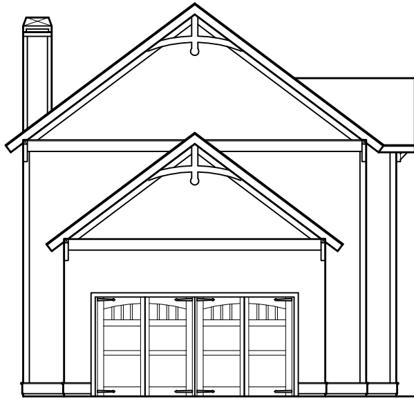
REAR ELEVATION
