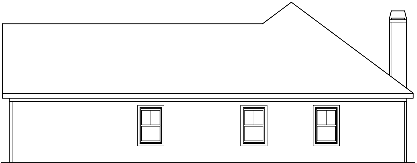
FRONT ELEVATION
