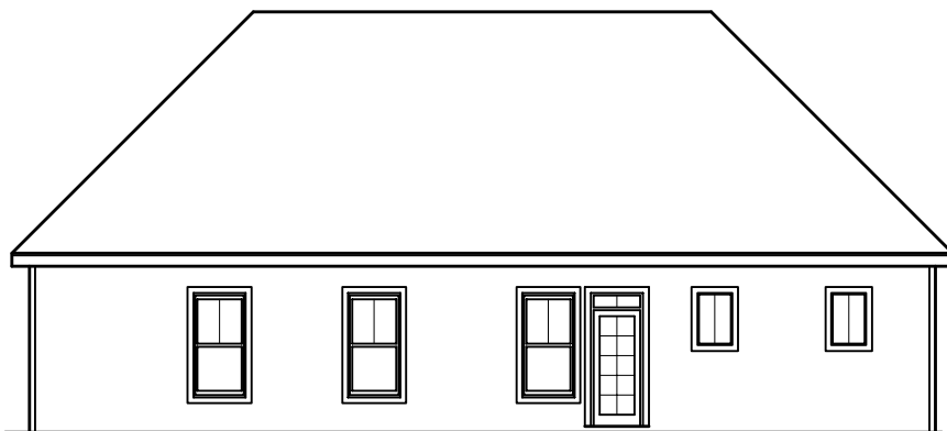
REAR ELEVATION
