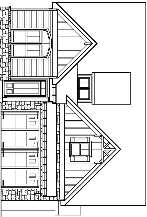
FRONT ELEVATION "A"
