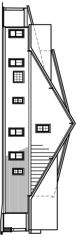
LEFT ELEVATION
