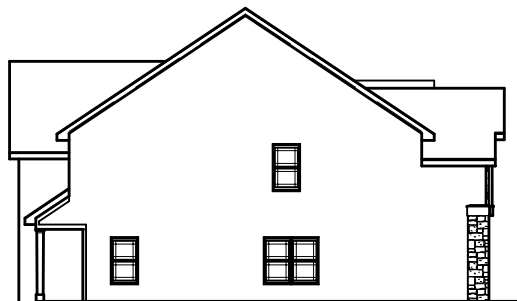
LEFT ELEVATION
